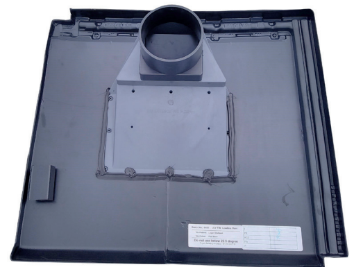
STR110: Square to round pipe adapter to suit 110mm flexi-pipe
