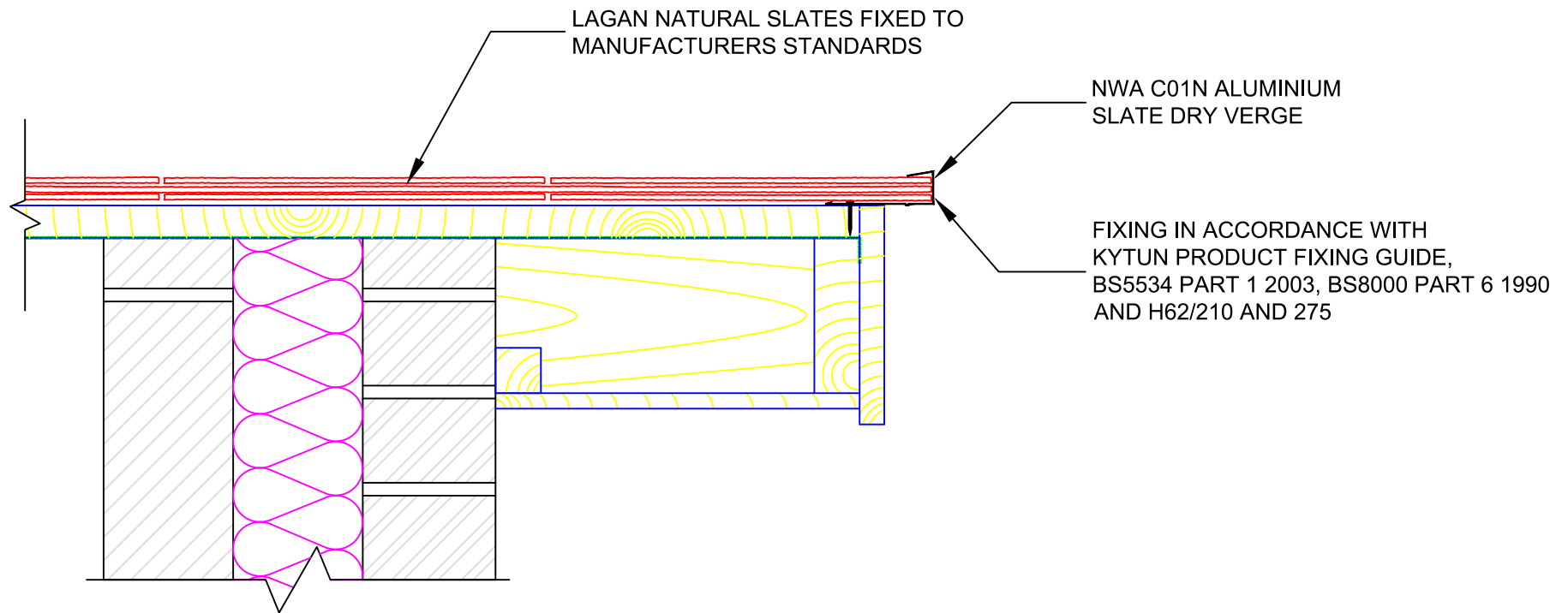
Lagan Natural Slate Verge Detail NWA C01N Aluminium Scale 1:5
